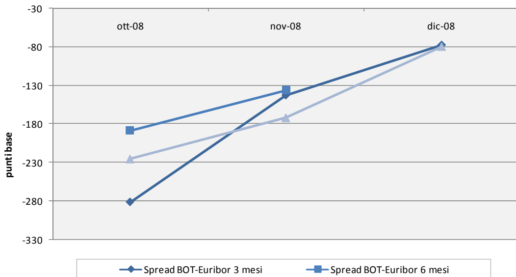
Figura B11: Spread Bot-Euribor
